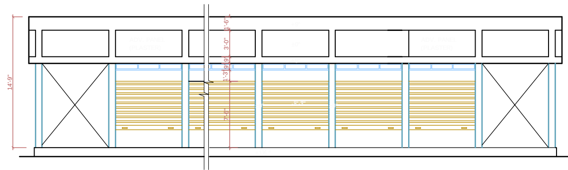
ELEVATION AT 2-2
