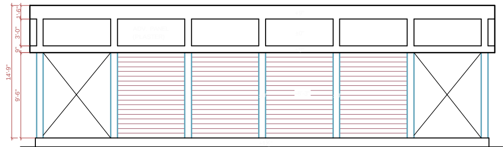
ELEVATION AT 1-1
